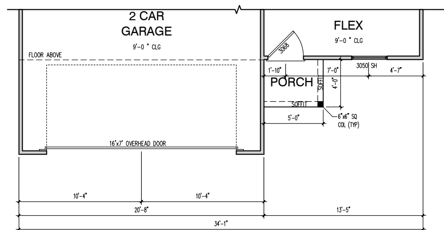
PARTIAL FIRST FLOOR PLAN SCALE 1/8" = 1'-0" (NOTE: SCALE 1/4" = 1'-0" ON 22x34 PAPER)
