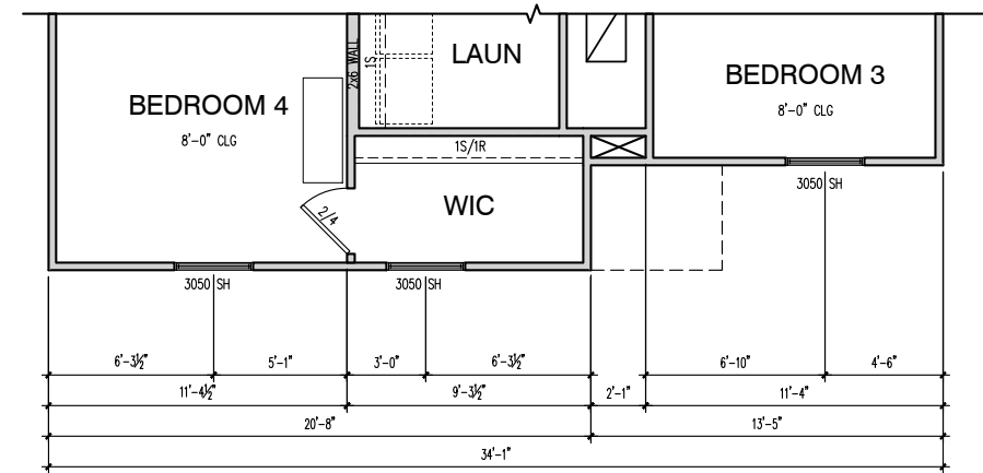
PARTIAL SECOND FLOOR PLAN
