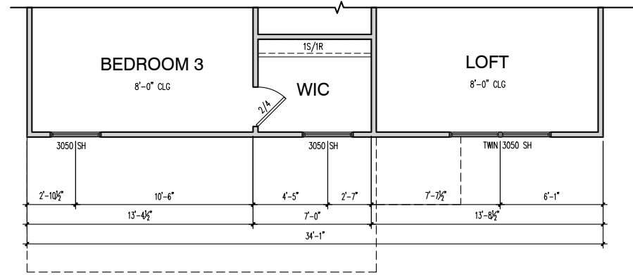
PARTIAL SECOND FLOOR PLAN SCALE 1/8" = 1'-0" (NOTE: SCALE 1/4" = 1'-0" ON 22x34 PAPER)
