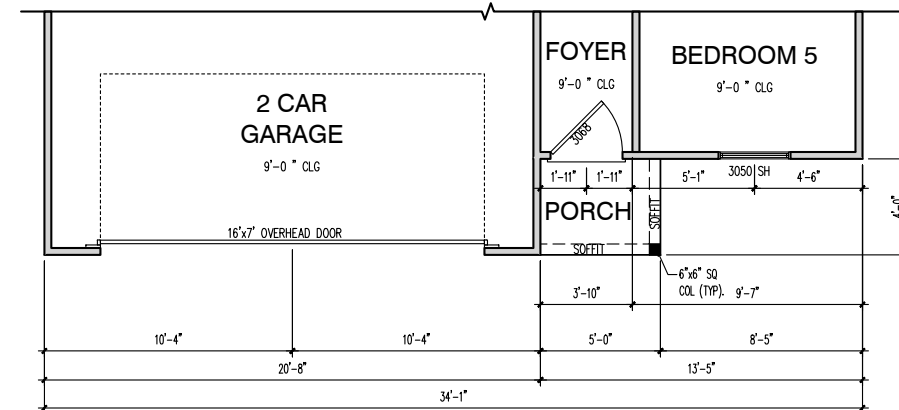
PARTIAL FIRST FLOOR PLAN
