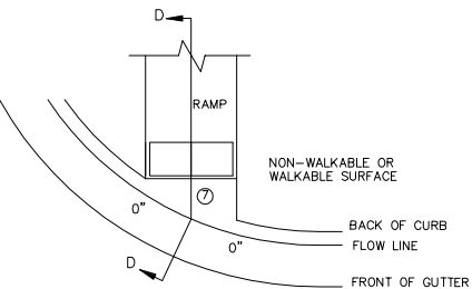
CURB FOR DIRECTIONAL RAMPS ⑬
