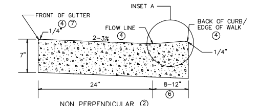
PEDESTRIAN ACCESS ROUTE CURB & GUTTER DETAIL
