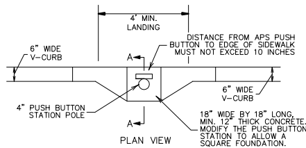
PLAN VIEW
