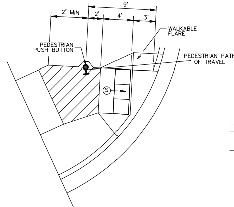
SEMI-DIRECTIONAL RAMP (3,4,9)
