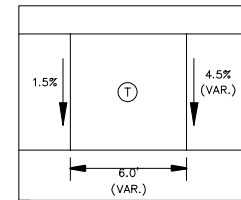
INSET A TRANSITION PANEL ④ ⑤
